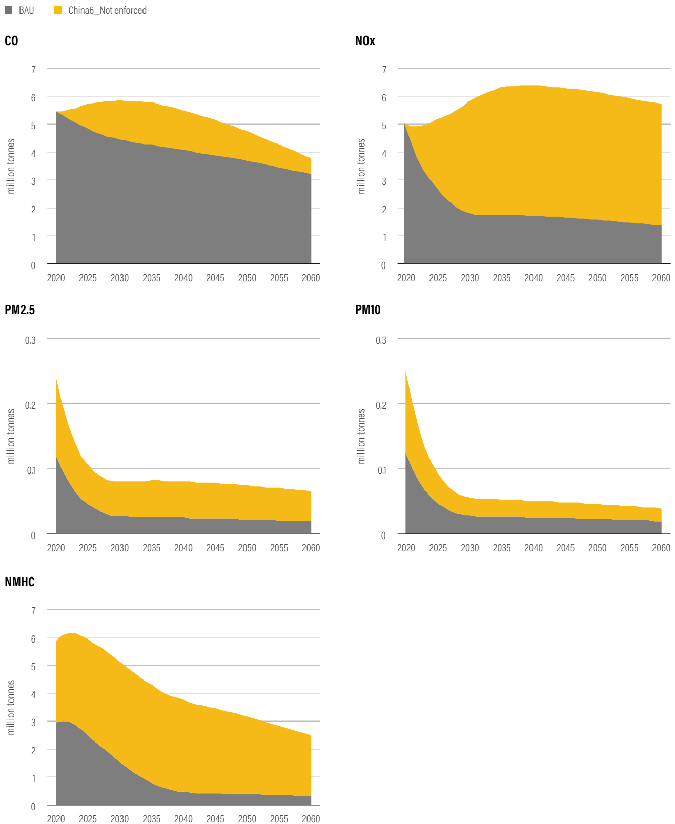
Figure 32 | Air Pollutant Reductions Resulting from the Introduction of China 6 Standard
